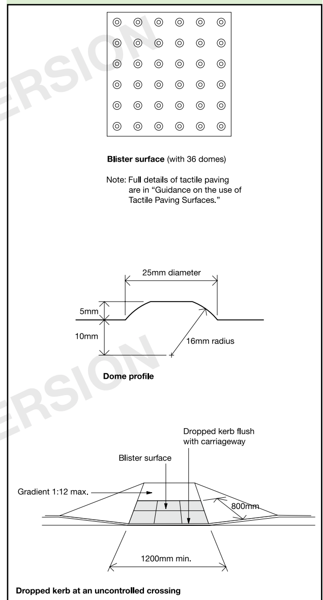
Diagram 1 Tactile paving and an example of its use at an uncontrolled crossing
