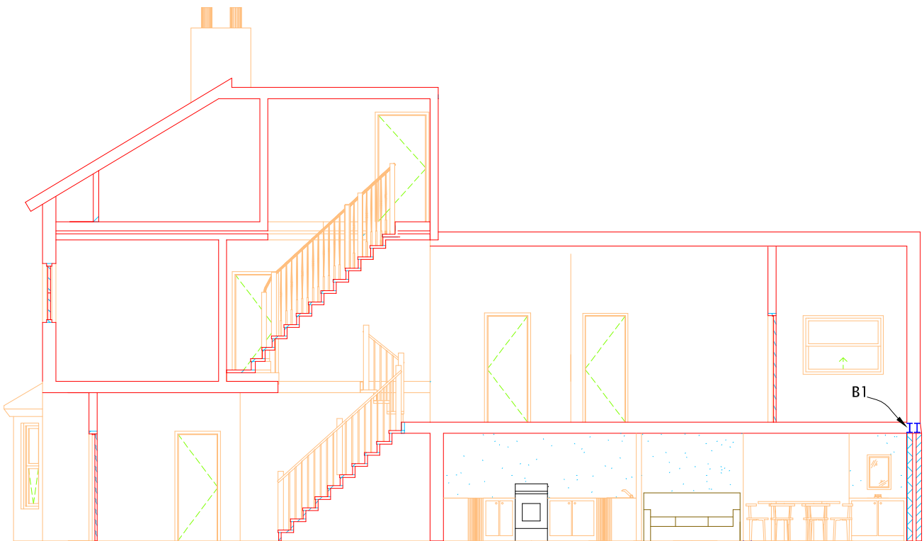
Section C-C
