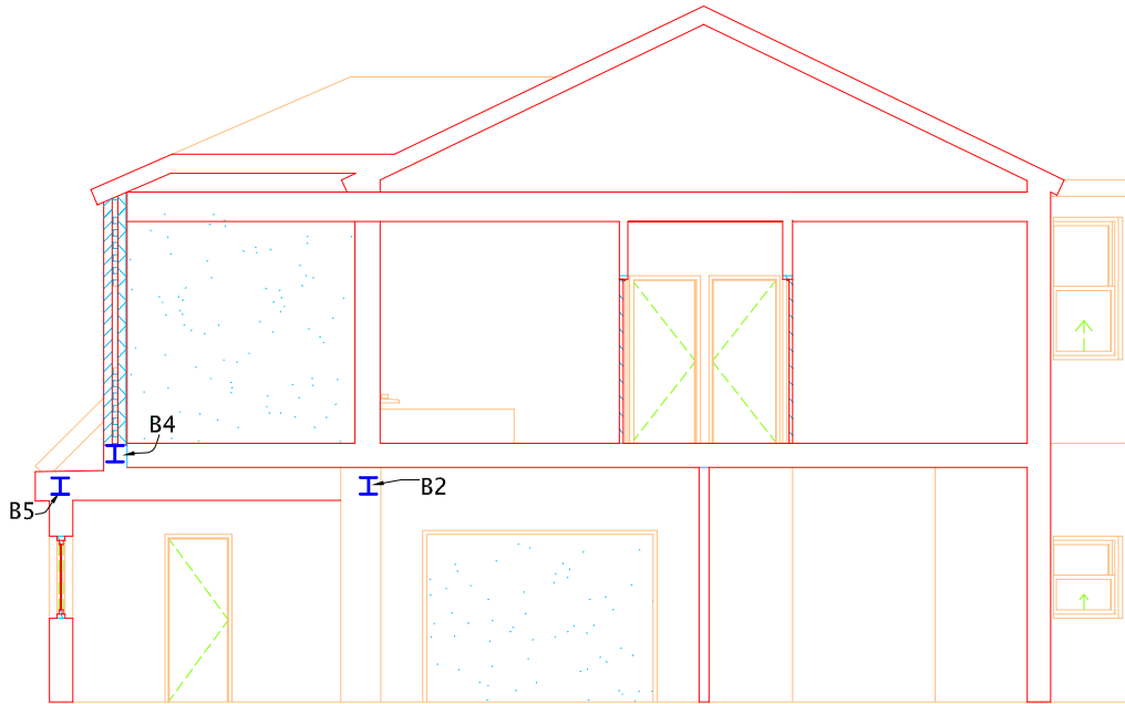
Section F-F
