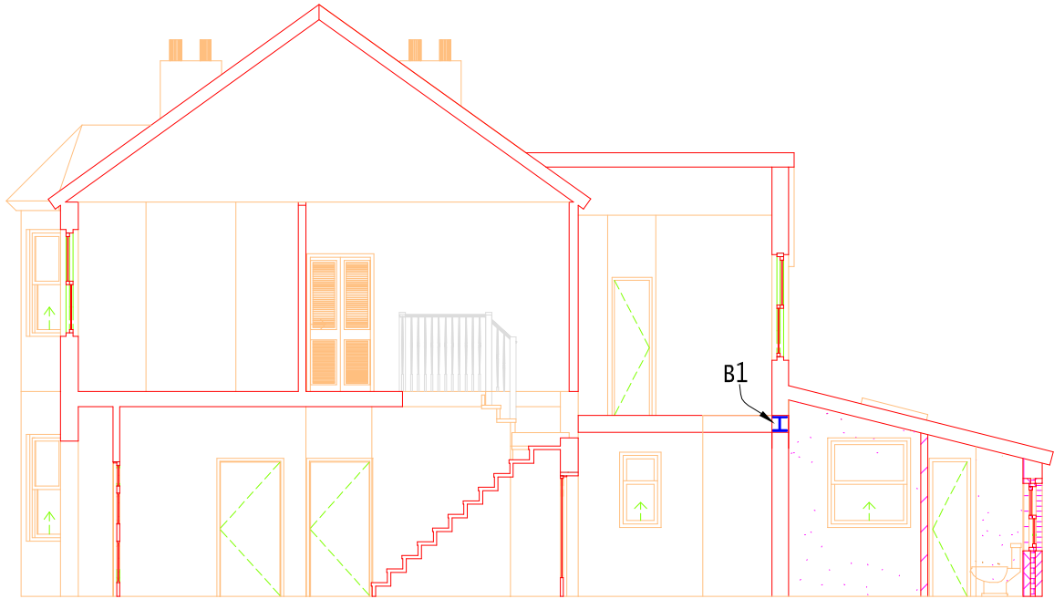
Section B-B
