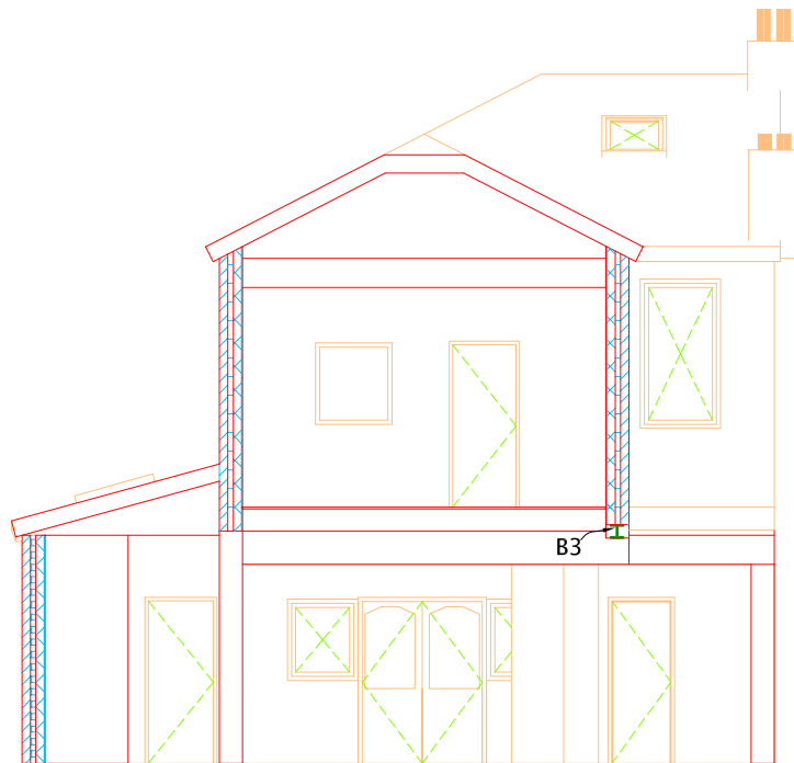
Section E-E
